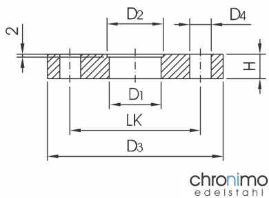
Glatter Flansch ND 10 flange plain ND 10
